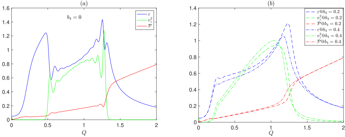
FIG. 3. (a) L H transition dynamics without noise. Notice that zonal flow exist only within the I-phase and residual turbulence exists in H-mode. (b) L H transition dynamics with noise. Notice that zonal flow exists at any power, but is most prominent within the I-phase. Noise eliminates the threshold for zonal flow appearance, increases the duration of I-phase, reduces the turbulence energy and reduces the ultimate power threshold for L H transition. Parameters are a_1 = 1 , a_2 = 0.2 , a_3 = 0.7 , a_4 = 0.7 , b_1 = 1.5 , b_2 = 0.7 , b_3 = 1 , c_1 = 1 , c_2 = 0.7 and c_3 = 0.5 .
