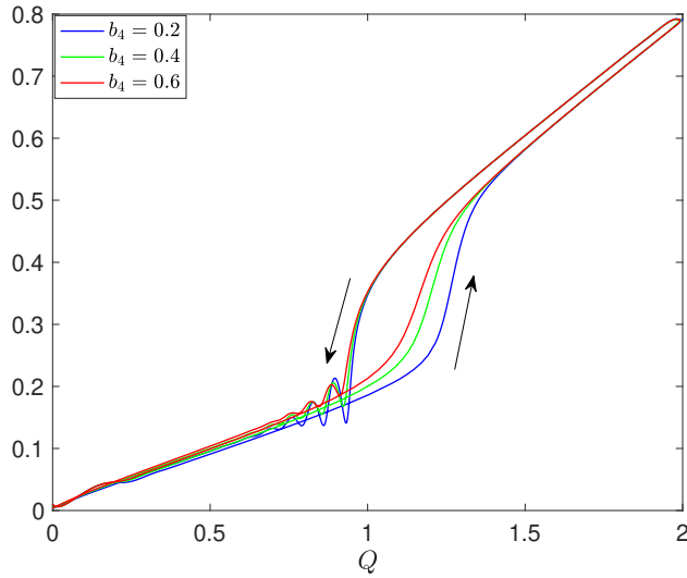
FIG. 5. Noise reduces the area enclosed in the hysteresis curve.
