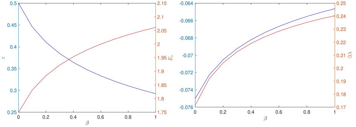
FIG. 2. Left: Stable fixed points with noise strength \beta . Zonal flow energy increases and turbulence energy decreases with \beta . Right: Eigenvalues \lambda of the stable fixed points.
