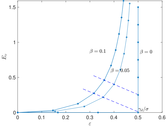
FIG. 1. Zonal flow energy E_v vs turbulence energy \varepsilon in a linear growth rate \gamma scan with noise strength \beta as a parameter.
