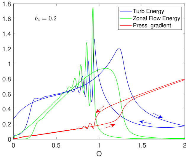
FIG. 4. The H-L back transition is accompanied by hysteresis. In presence of zonal noise, hysteresis is robust with respect to variations in initial conditions and the point of retreat (in Q ) in the H mode.
